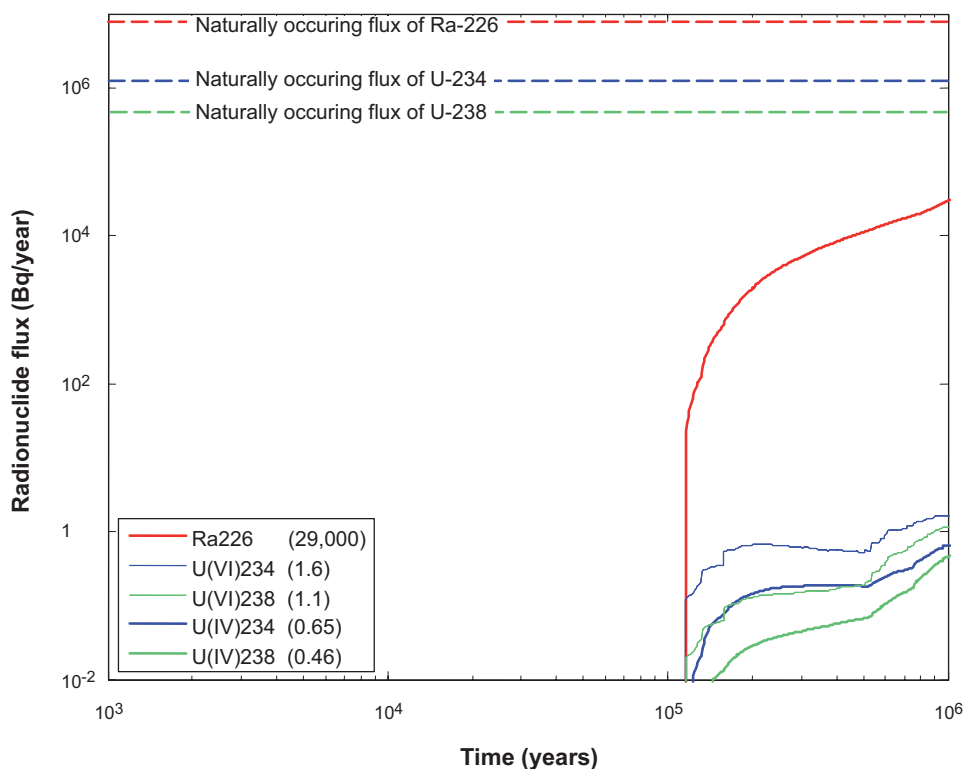
Figure S-14. Far-field release rates (Bq/year) of U-238, U-234 and Ra-226 in the central corrosion case compared to the naturally occurring fluxes at Forsmark.
