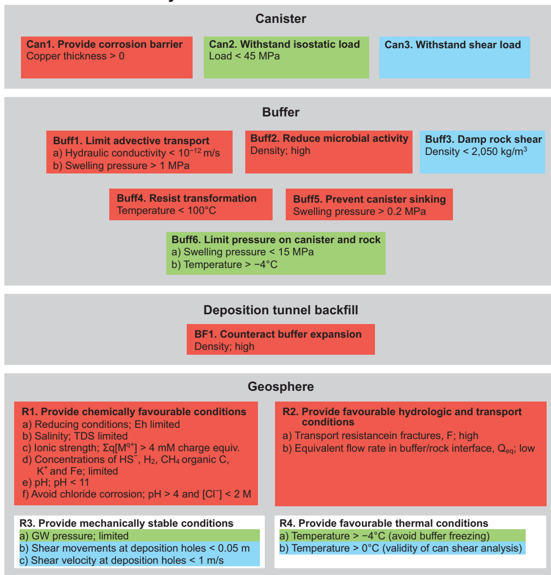
Figure S-7. Safety functions (bold), safety function indicators and safety function indicator criteria related to containment. When quantitative criteria cannot be given, terms like “high”, “low” and “limited” are used to indicate favourable values of the safety function indicators. The colour coding shows how the functions contribute to the canister safety functions Can1 (red), Can2 (green) and Can3 (blue).
