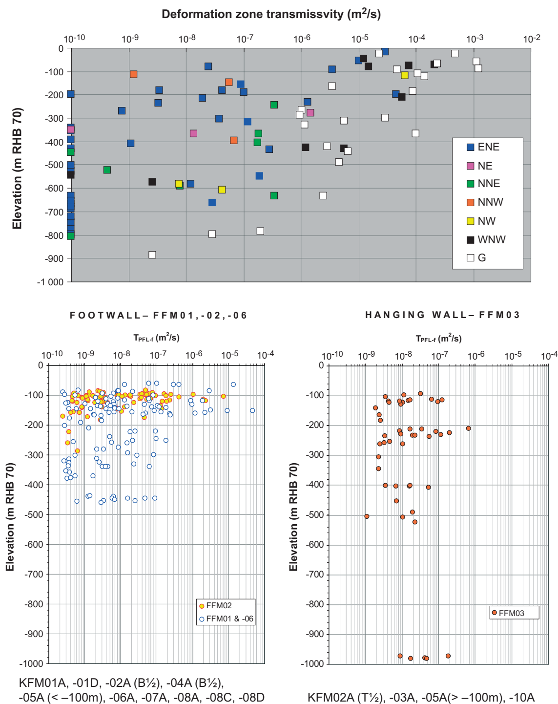
Figure 4-16. Top: Inferred transmissivities of deformation zones with depth and orientation (G = gently dipping zones). Bottom: Inferred transmissivities of connected open fractures with depth in FFM01, FFM02 and FFM06 (left) and FFM03 (right) (Figure 11-19 in the Site description Forsmark ). Note that the bottom left insert contains data from 10 boreholes whereas the bottom right insert contains data from 4 boreholes only (B½ = bottom half of the borehole, T½ = top half of the borehole).
