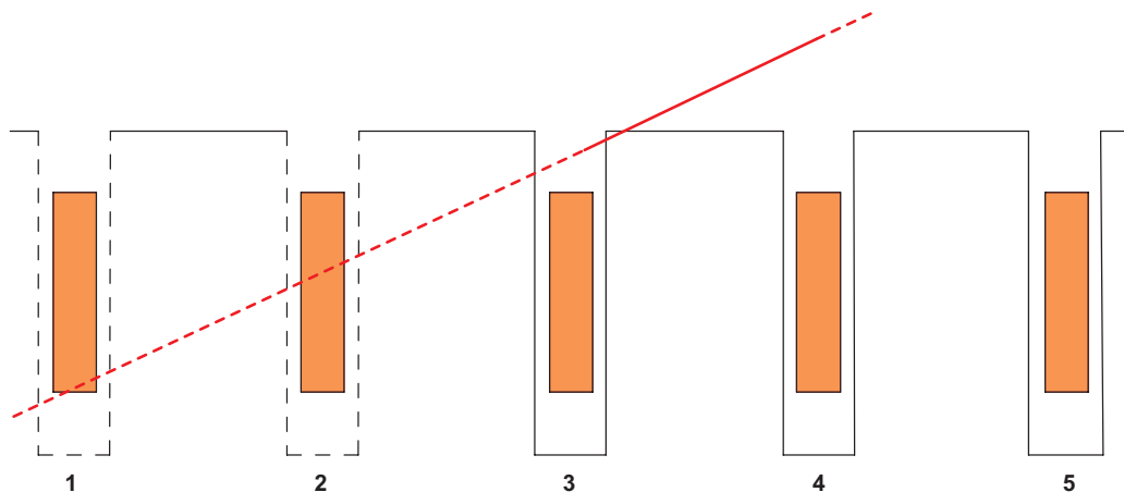
Figure 5-4. In SR-Site, the EFPC criterion is changed such that deposition positions being intersected by a fracture that intersects the full tunnel perimeter and that also is projected to intersect the canister location in the deposition hole, are rejected (i.e. positions 1 and 2). For potentially water bearing fractures the previous criterion still applies (i.e. position 3 is also rejected).
