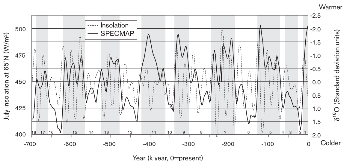
Figure 6-2. \delta^{18}\text{O} variation from five drill cores of deep sea sediments expressed as number of standard deviations from the long-term mean. From /Imbrie et al. 1984/. \delta^{18}\text{O} variations reflect the temperature of the sea and the volume of water that has been bound in land-based ice sheets and glaciers all over the world. The grey and white fields indicate warm and cold periods.
