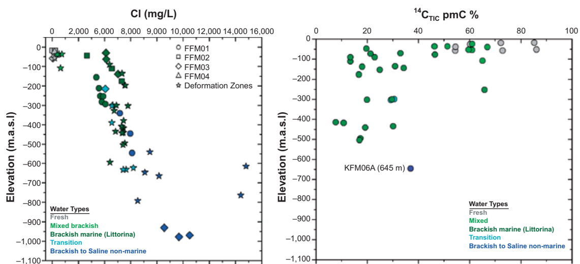
Figure 4-21. Left: Cl - concentration as a function of elevation as measured in groundwater from the different fracture domains and from deformation zones (from Figure 9-5 in the Site description Forsmark ). Right: 14 C TIC as a function of elevation. The only sample of brackish non-marine groundwater type analysed indicated contamination during sampling (Figure 9-20 in the Site description Forsmark ).
