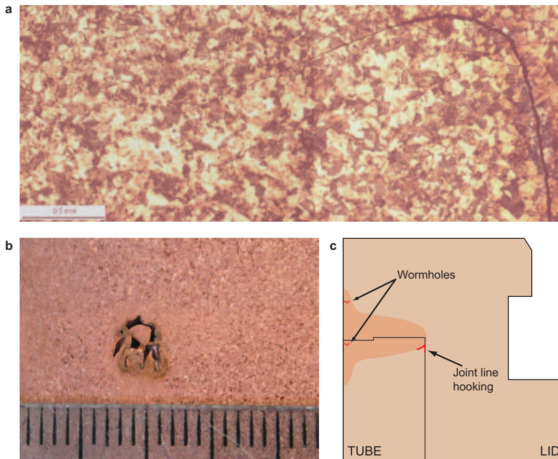
Figure 5-10. a) Photograph of joint line hooking (from /SKBdoc 1175162/). b) Photograph of wormhole (from /SKBdoc 1175162/). Schematic cartoon showing positions of defects in friction stir welds (redrawn from the Canister production report ).
