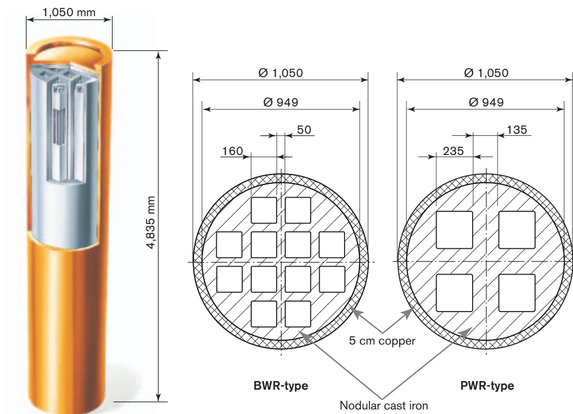
Figure S-5. Left: The reference design with a corrosion resistant outer copper shell and a load-bearing insert of nodular cast iron. Right: Cross section of insert designs of the BWR and PWR types.
