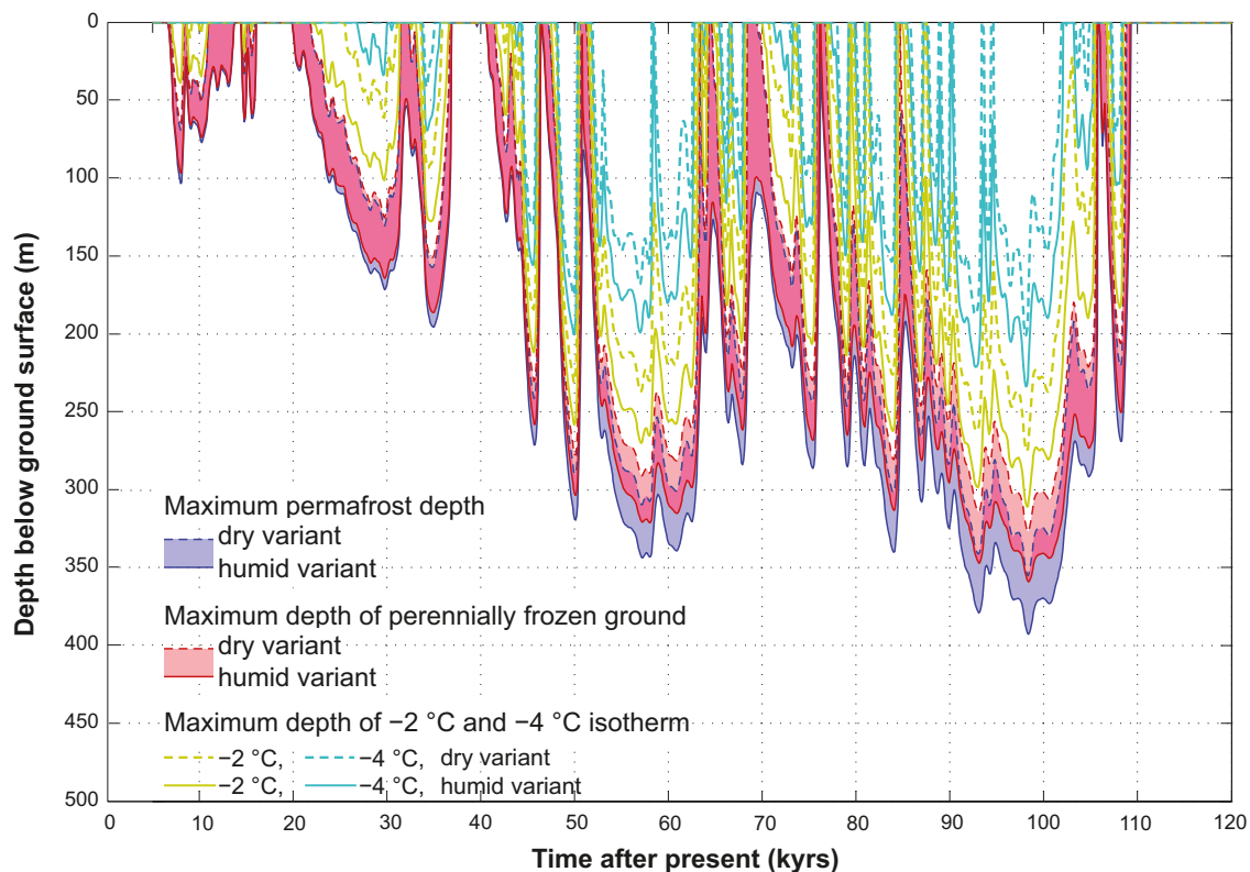
Figure 7-11. Evolution of maximum permafrost depth, maximum depth of perennially frozen ground and maximum depth of -2 and -4^{\circ}\text{C} isotherms over the repository for the Severe permafrost case. The shaded areas in blue and red represent the range when considering the dry and humid climate variants of the Severe permafrost case. The darker lilac colour indicates that the results for permafrost and perennially frozen ground overlap. Reproduced from figure 5-24 of the Climate report .
