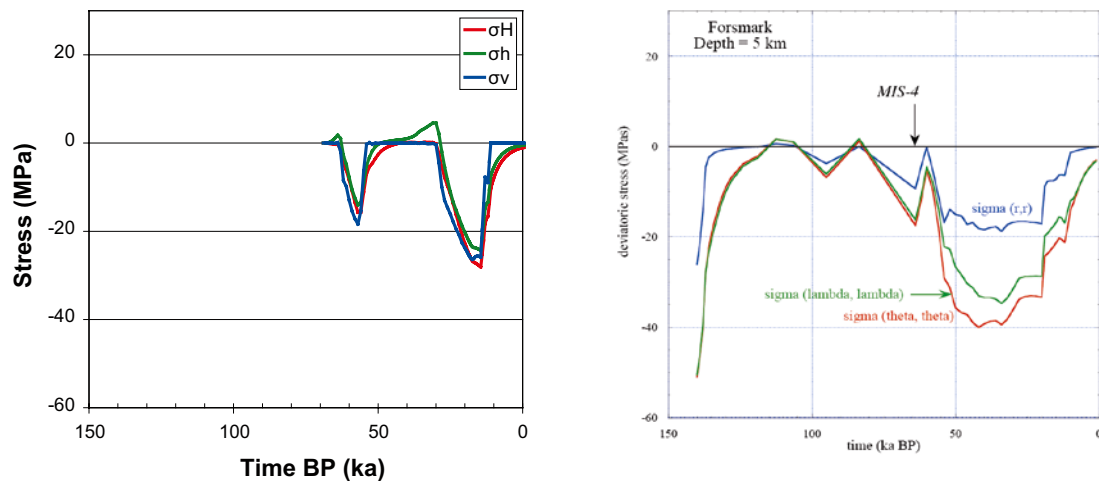
Figure 6-26. Left: Temporal evolution of the glacially induced stresses (model T9) at 5.5 km depth obtained from ice-crust-mantle analyses performed by /Lund et al. 2009/ using Näsland's /SKB 2006c/ ice model. Right: Modelled stresses at 5 km depth due to Lambeck's ice model, reproduced from /Lambeck 2005, Figure 7/. Here, compression is negative. The scale of the right figure is the same as in the left figure.
