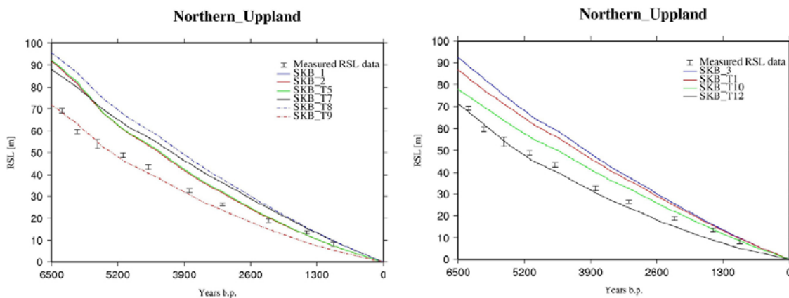
Figure 6-28. Comparison between measured relative sea-level data in northern Uppland and model results from flat layered Earth models (left) and Earth models with variable layer thickness (right). Excerpt from /Lund et al. 2009, Figure 6-7/.
