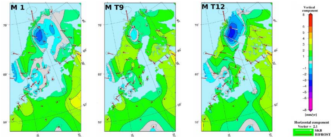
Figure 6-27. Comparison between data from the Bifrost project (GPS data) and model results. Contours show differences in vertical velocities, whereas arrows show horizontal velocity components from the Bifrost project (red) and model results (white). Reproduced from /Lund et al. 2009, Figures 6-2, 6-3, and 6-5/.
