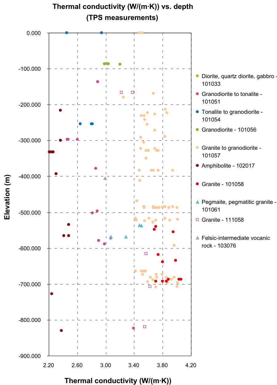
Figure 6-9. Thermal conductivity versus elevation for different rock types. Samples measured using the TPS method. Reproduced from /Back et al. 2007, Figure 3-1/.
