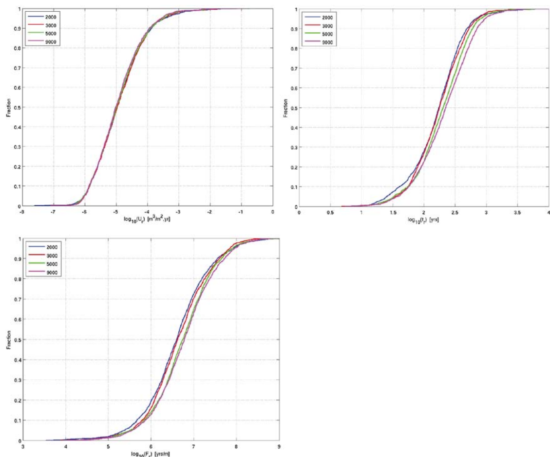
Figure 6-67. Normalised CDF plots of Darcy flux q (denoted U_r in figure caption,) t_w and F (denoted t_n and F_r in figure captions to indicate that t_w and F are calculated in the bedrock described as a DFN only) in the Hydrogeological base case model at 2000 AD, 3000 AD, 5000 AD, and 9000 AD for release path Q1. The t_w and F_r plots are based on particles successfully reaching the model top boundary (cf. /Selroos and Follin 2010, Figure 5-9/).
