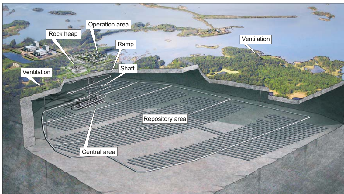
Figure 2-4. The central area of the repository with ramp and shaft /SKB 2010f/.
