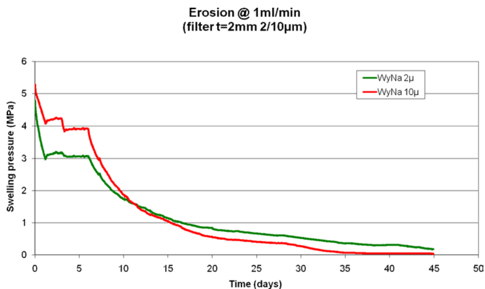
Figure 3-30. Swelling pressure for Wy-Na montmorillonite as a function of time using filter pore sizes of 2 and 10 \mu m respectively. The drop in swelling pressure is caused by loss of clay through the filters (2 mm thick). /Birgersson et al. 2010, Hedström et al. 2011/.
