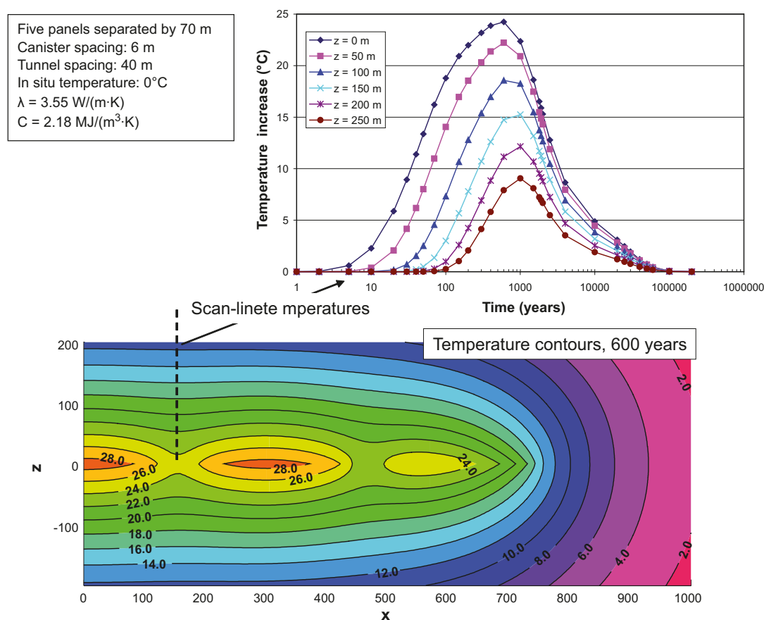
Figure 6-1. Example of contours of temperature increase (lower) and temperature increases on vertical scan-lines between deposition areas (upper). Results obtained using the method described in /Hökmärk et al. 2009/.
