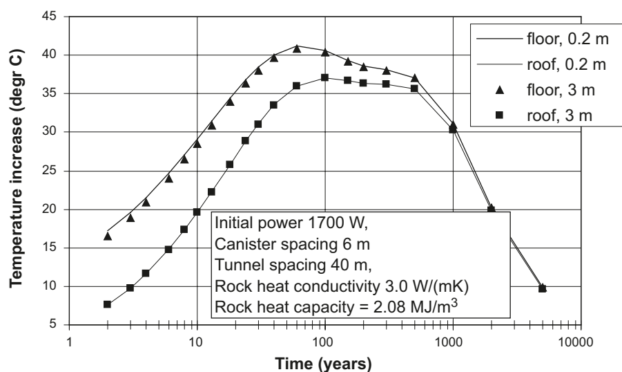
Figure 4-1. Temperatures in tunnel floor and tunnel roof for two positions: 0.2 m and 3 m, respectively, from the axis of the nearest canister. Temperatures are calculated with an analytical solution given by /Claesson and Probert 1996/ without regard to the properties of the backfill.
