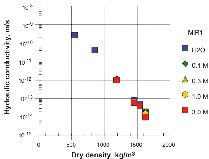
Figure 3-6. Hydraulic conductivity of Deponit CaN(MiR1) bentonite measured at different densities and molar concentration of CaCl₂ in the saturating solution /Karnland et al. 2006/.
