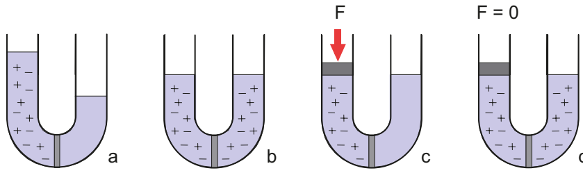
Figure 3-19. The basic principles of osmosis as an analogy of bentonite swelling pressure /Karnland et al. 2005/.
