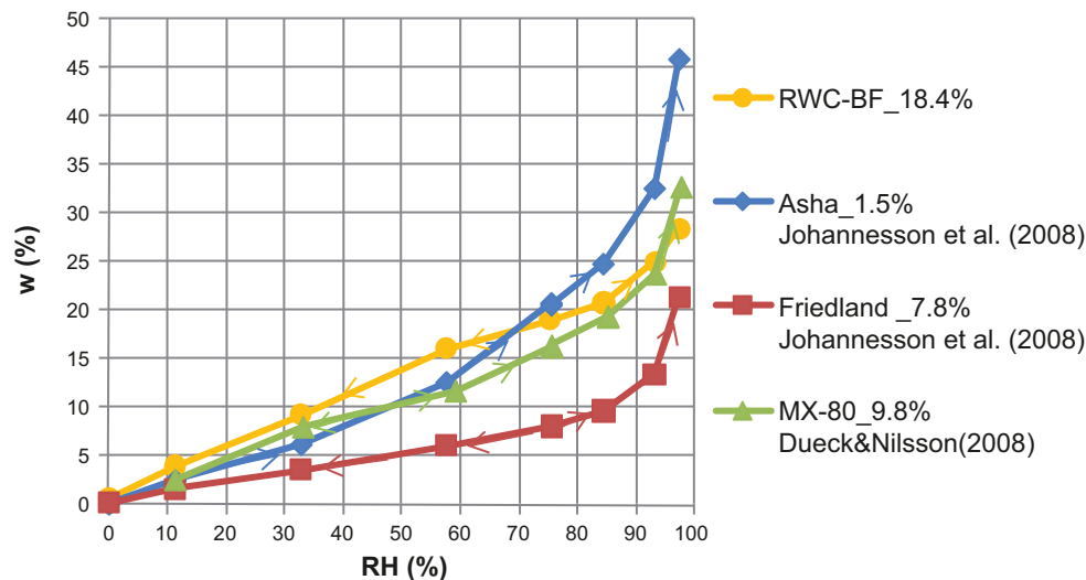
Figure 4-2. Specific retention curve for the RWC-BF material obtained at 25°C shown together with previous results for Asha and Friedland at 25°C and MX-80 at 20°C. The labels show material and initial water content (%). The arrows show the moisture paths /Johannesson et al. 2010/.
