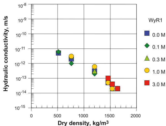
Figure 3-5. Hydraulic conductivity of MX-80(WyR1) bentonite measured at different densities and molar concentration of NaCl in the saturating solution /Karnland et al. 2006/.
