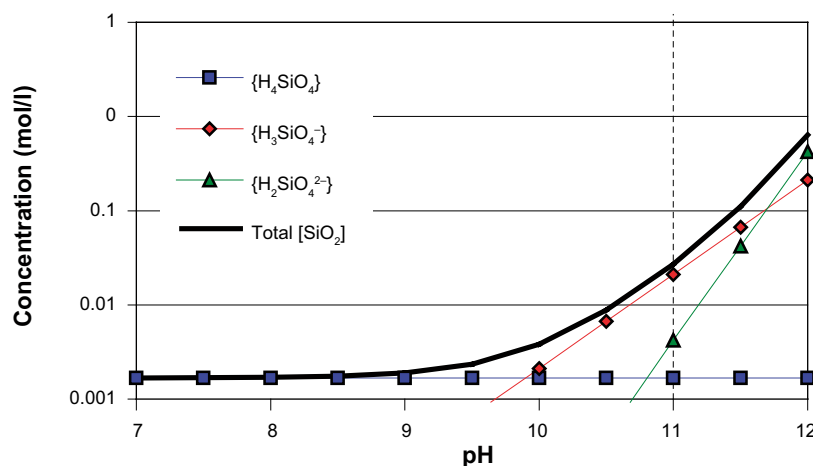
Figure 3-26. Total concentration of silica as a function of pH assuming \text{H}_4\text{SiO}_4 activity for saturated amorphous silica at 25°C. At pH=9.9 \text{H}_3\text{SiO}_4^- starts to dominate and above pH=11.7 \text{H}_2\text{SiO}_4^{2-} dominates. The upper limit for the KBS-3 design criterion, pH=11, is indicated /Karnland et al. 2006/.
