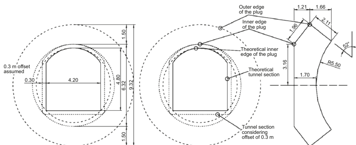
Figure 7-2. Dimensions of the concrete plug.
