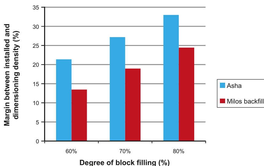
Figure 4-5. Margin between the installed and dimensioning density for Milos backfill and Asha at different block parts of the tunnel volume. Dimensioning density for Asha 1,160 kg/m 3 from /Gunnarsson et al. 2006/.
