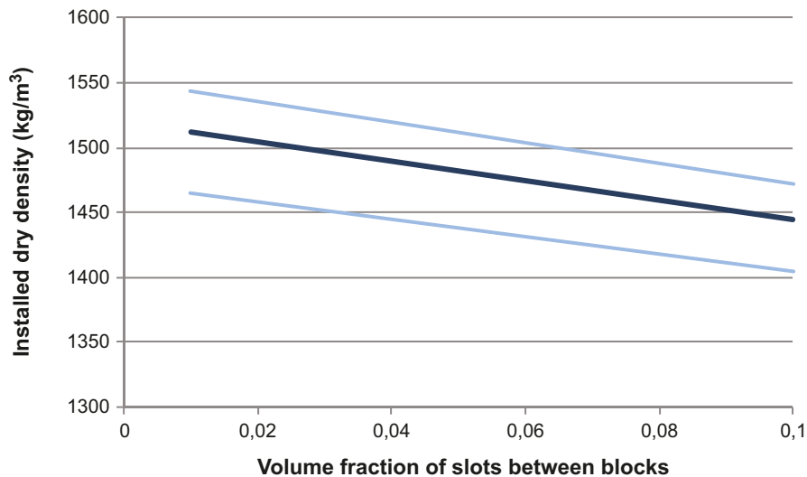
Figure 6-2. The installed dry density as a function of the volume fraction of the slots between the blocks in the block masonry. The installed dry density is calculated for the average tunnel volume (dark blue line) and the smallest and largest expected tunnel volumes (light blue lines).
