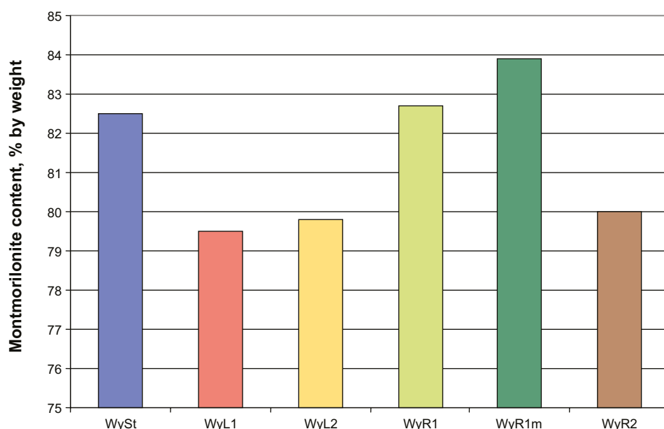
Figure 5-5. Results of X-ray diffractation inspections and analysis of diffractation patterns showing the montmorillonite content in the five consignments representing over 20 years of production of MX-80 bentonite /Karnland et al. 2006/. The Stripa (WySt) material represents material delivered around 1980, and the others were delivered 1995 (WyL1), 1999 (WyL2), and 2001 (WyR1 and WyR2).
