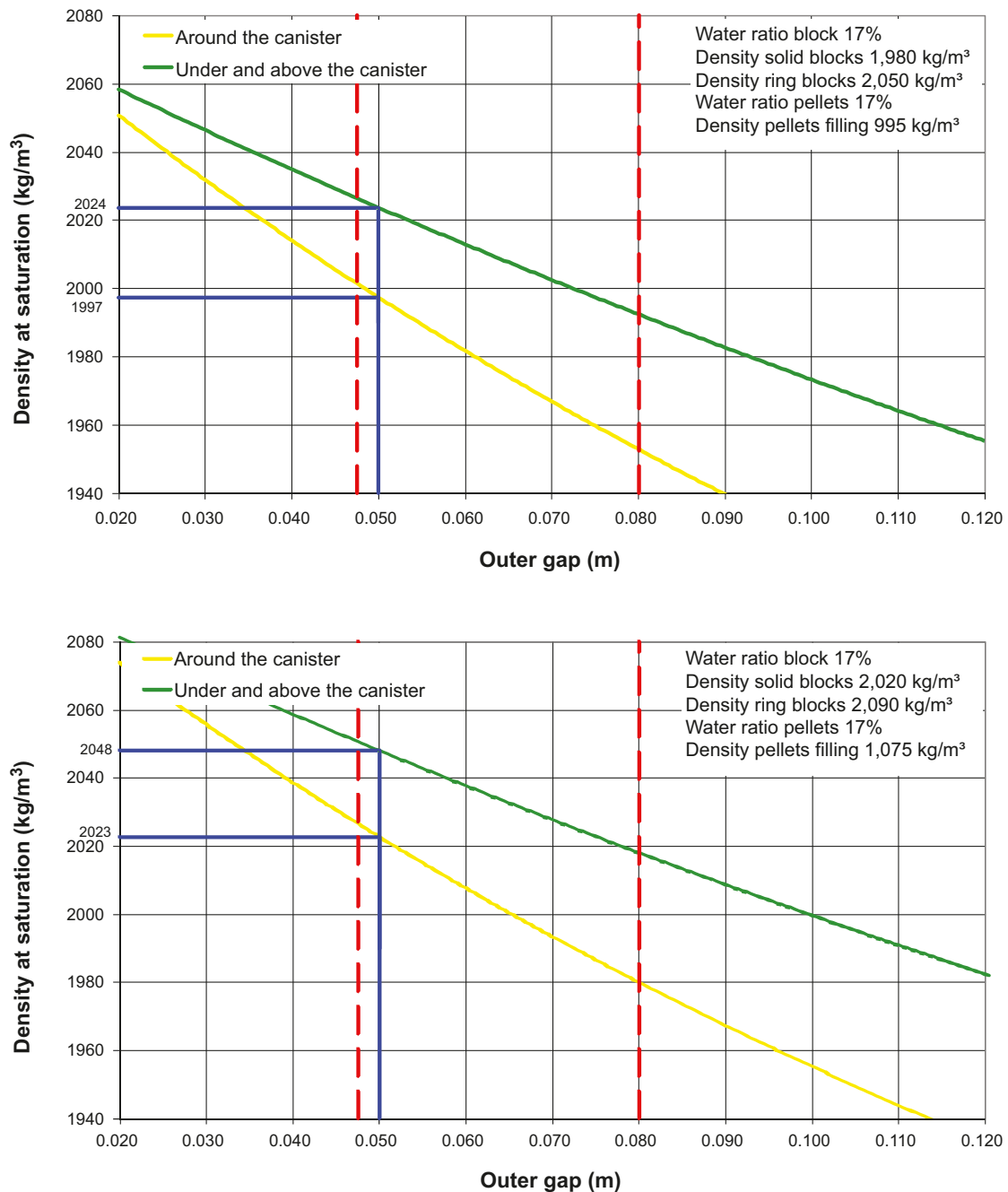
Figure 4-8. The calculated saturated density of the buffer as function of the width of the pellet filled gap between the bentonite blocks and the wall of the deposition hole. Upper panel: Assuming minimum density of the buffer blocks and pellets. Lower panel: Assuming maximum density of blocks and pellets. (Blue line: nominal gap.) The red dotted lines illustrate the maximum accepted area of the cross section which exceeds the nominal with 7.0%.
